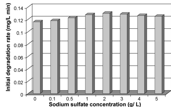
Fig. 13. Effect of sodium sulfate addition on sonochemical degradation of RhB (conditions: volume: 300 mL; initial dye concentration: 5\text{ mg L}^{-1} ; temperature: 25\text{ }^\circ\text{C} ; pH: 5.3; frequency: 300 kHz; power: 60 W).
